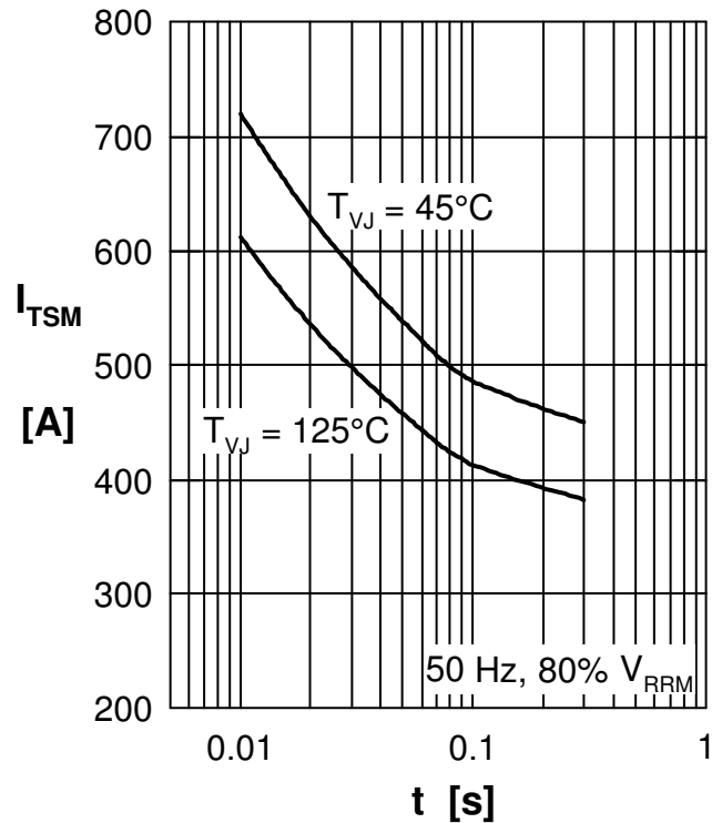
Fig. 2 Surge overload current
