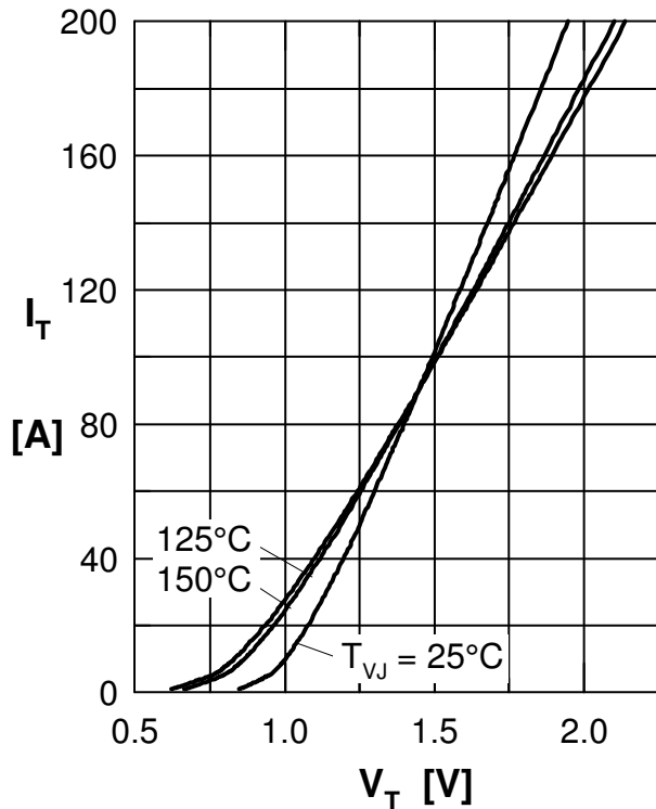
Fig. 1 Forward characteristics
