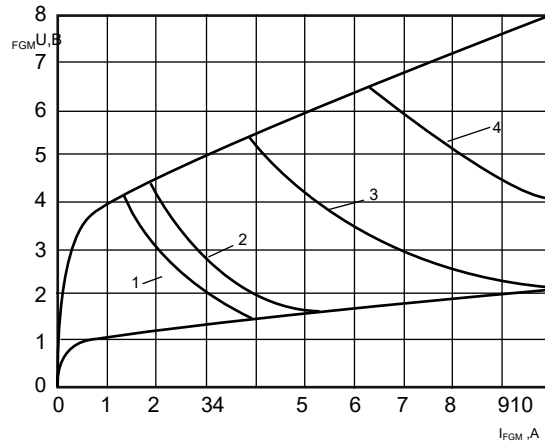
Fig.7 Gate characteristic
